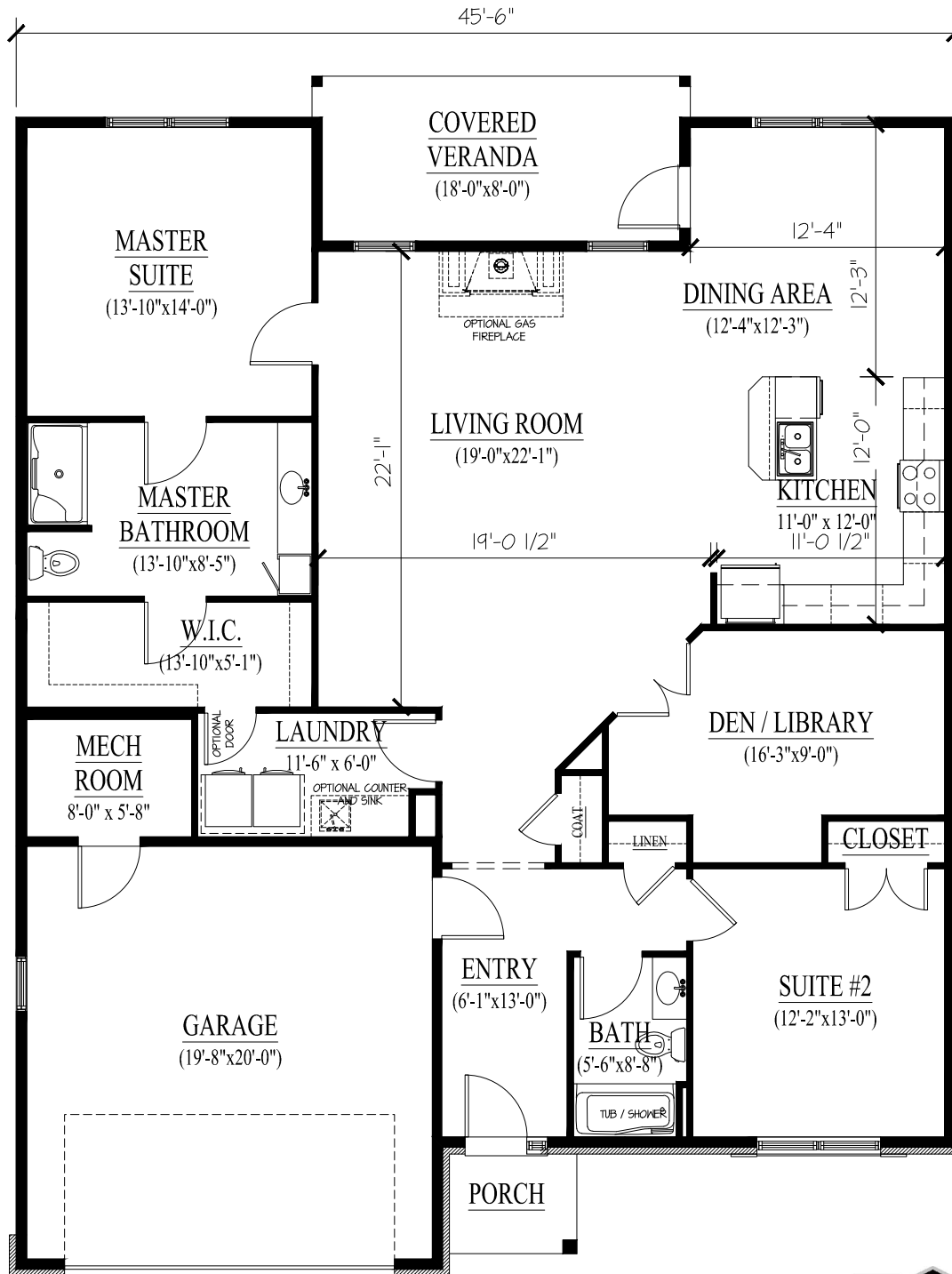
FIRST FLOOR PLAN 1882 SQ.FT.
